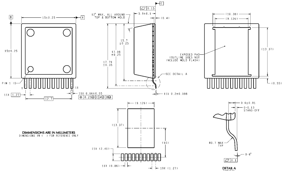
RECOMMENDED LAND PATTERN 11-Lead TZA Package NS Package Number TZA11A
