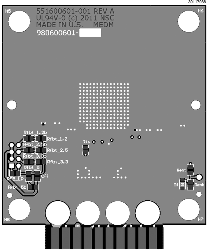
FIGURE 5. Layout Example
