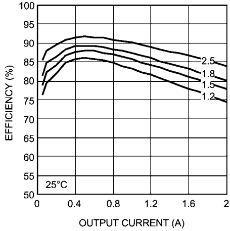
Efficiency 6V Input @ 25°C
