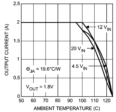
Thermal Derating V OUT = 1.8V
