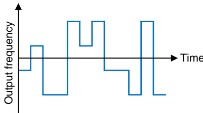
Figure 25. FSK Modulation
