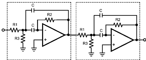
FIGURE 4. Active Filter
