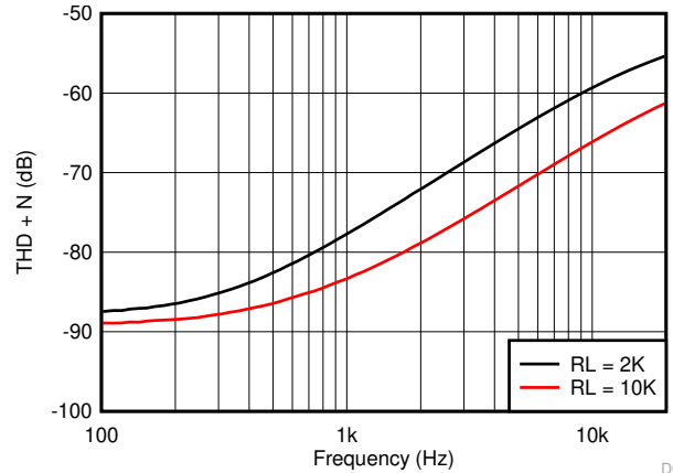
Figure 6-14. THD + N vs Frequency V_S = 5.5\text{ V}, V_{CM} = 2.5\text{ V}, G = 1, BW = 80\text{ kHz}, V_{OUT} = 0.5\text{ V}_{RMS}
