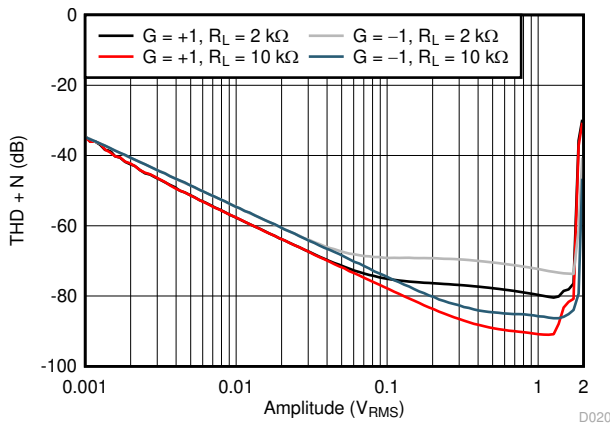
Figure 6-15. THD + N vs Amplitude V_S = 5.5\text{ V}, V_{CM} = 2.5\text{ V}, f = 1\text{ kHz}, G = 1, BW = 80\text{ kHz}
