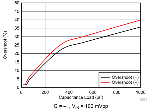
Figure 6-20. Small Signal Overshoot vs Capacitive Load
