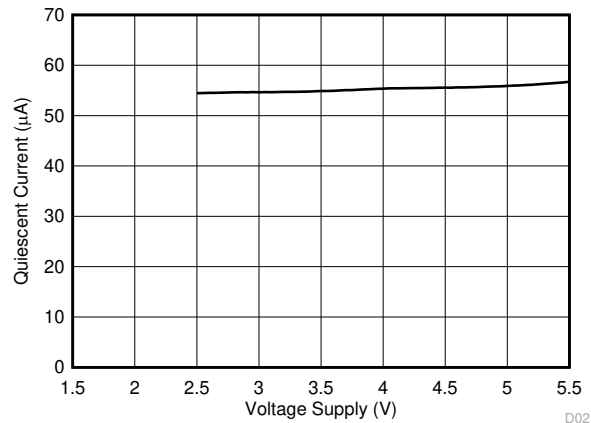
Figure 6-16. Quiescent Current vs Supply Voltage
