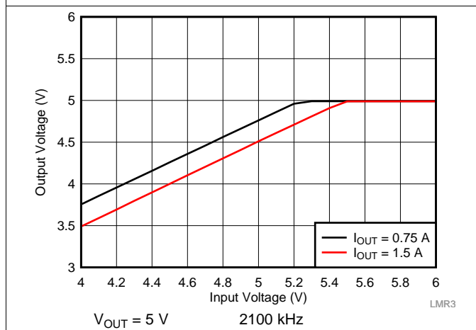
Figure 38. Overall Dropout Characteristic
