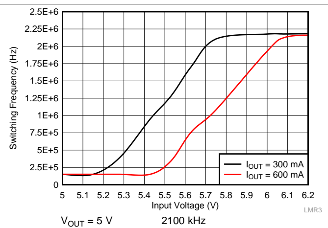
Figure 39. Frequency Dropout Characteristic
