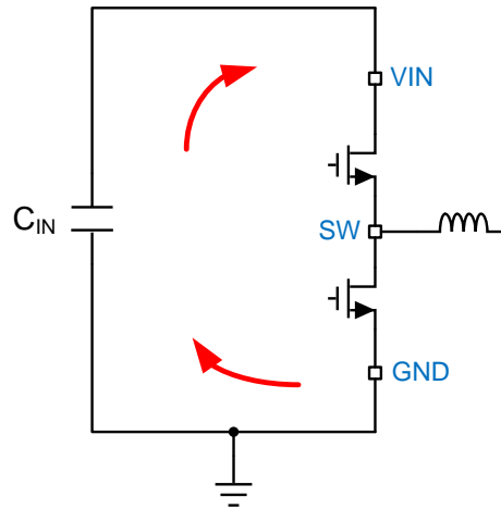
Figure 43. Current Loops with Fast Edges
