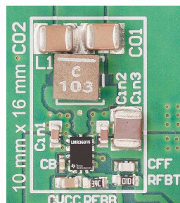
Typical PCB Layout
