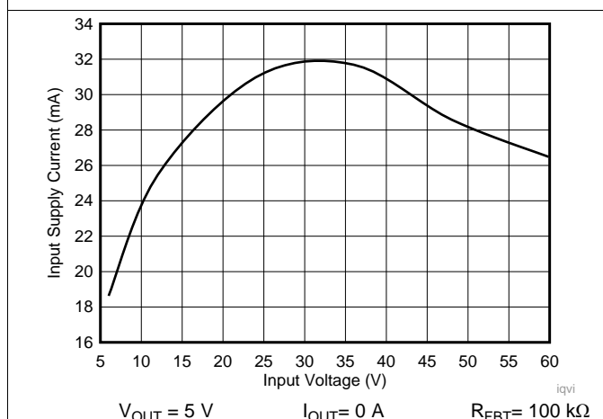
Figure 40. Input Supply Current
