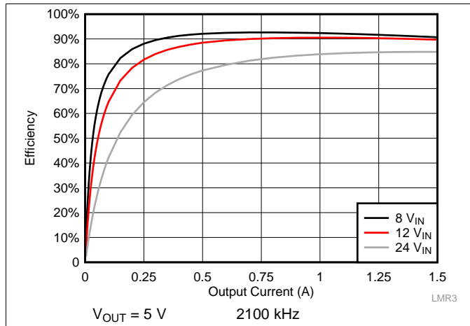
Figure 36. Efficiency
