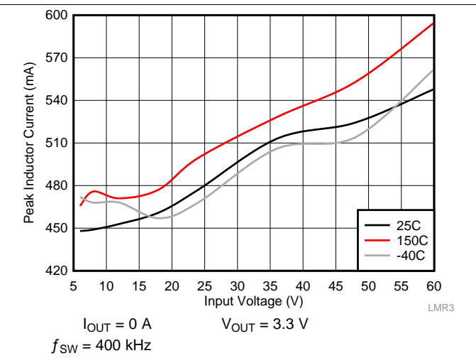
Figure 6. I PEAK-MIN
