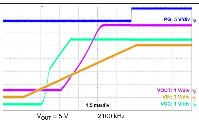
Figure 41. Start-Up Waveform
