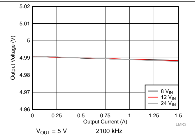
Figure 37. Load Regulation
