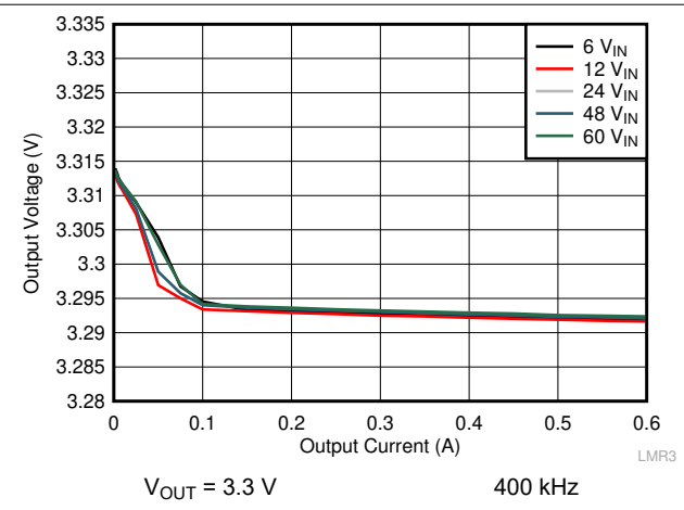
Figure 9-8. Load Regulation
