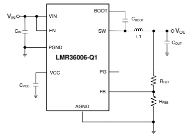
Simplified Schematic
