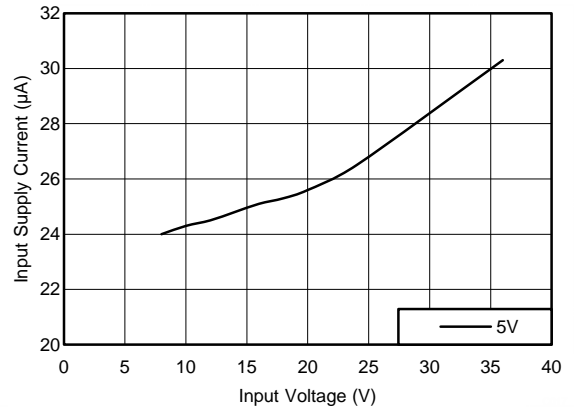
Figure 36. Input Supply Current
