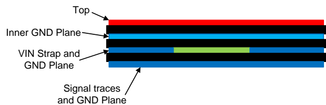
Figure 50. Example Layout for VQFN Package
