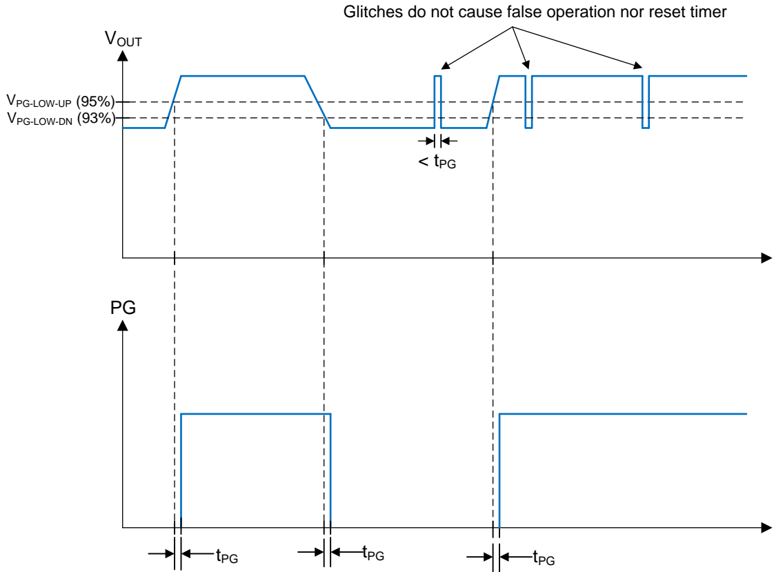
Figure 8. Power-Good-Timing Behavior
