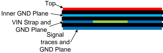
Figure 44. Example Layout for VQFN Package
