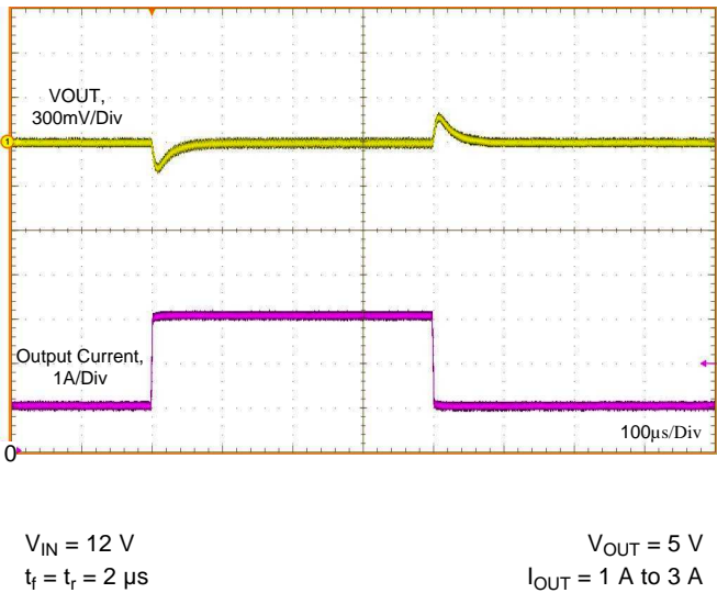
Figure 35. Load Transient
