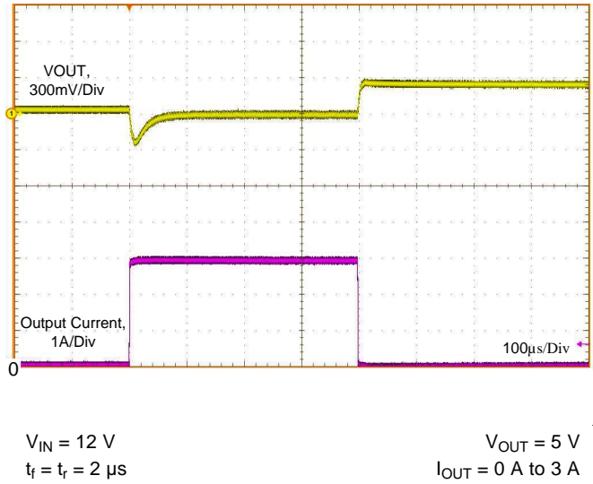
Figure 34. Load Transient
