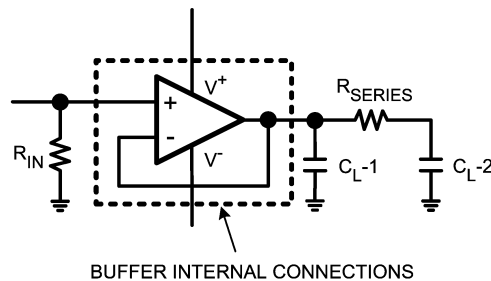
BUFFER INTERNAL CONNECTIONS
