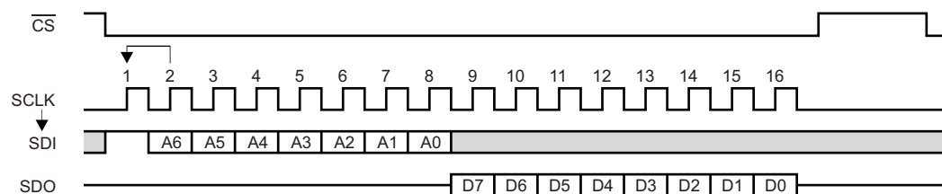
Figure 46. SPI Read Bus Cycle Timing Diagram
