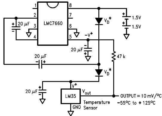
FIGURE 11. \mu Power Thermometer Spans 180^\circ C , and Pulls Only 150 \mu A
