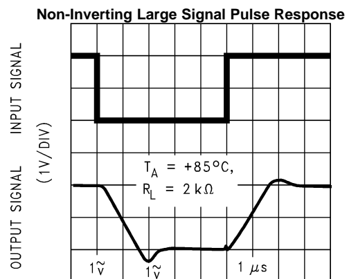
TIME (1 \mu s /DIV) Figure 55.
