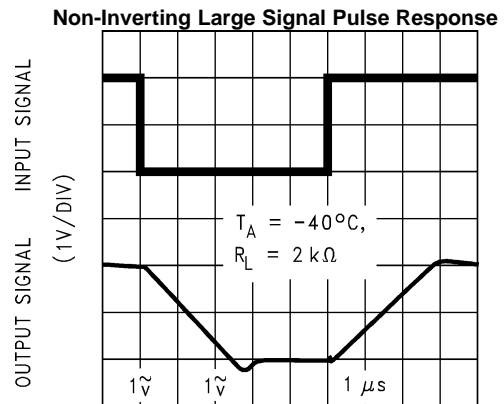
TIME (1 \mu s /DIV) Figure 53.
