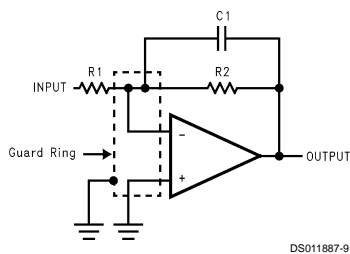
Inverting Amplifier
