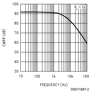
Common Mode Rejection Ratio vs Frequency
