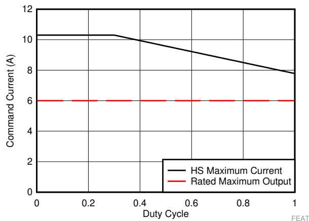
Figure 20. Maximum Current Allowed Through the HS FET - Function of Duty Cycle for LM61460-Q1
