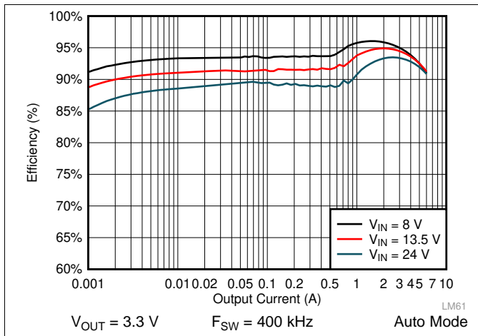
Figure 35. LM61460-Q1 Efficiency
