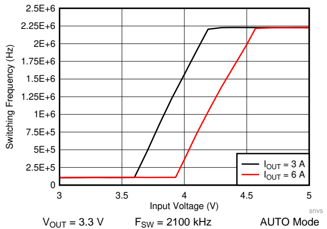
Figure 56. LM61460-Q1 Frequency Dropout Curve
