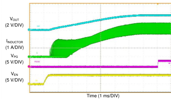
Figure 61. LM61460-Q1 Start Up with 50-mA Load
