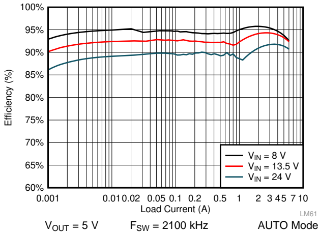
Figure 41. LM61460-Q1 Efficiency
