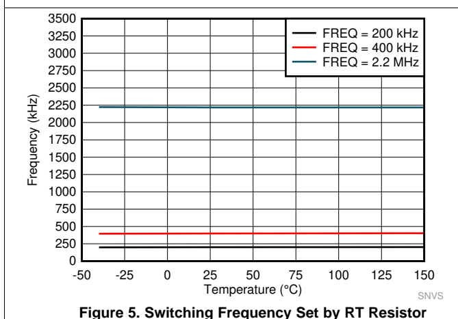
Figure 5. Switching Frequency Set by RT Resistor
