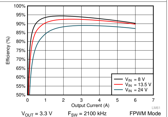
Figure 38. LM61460-Q1 Efficiency
