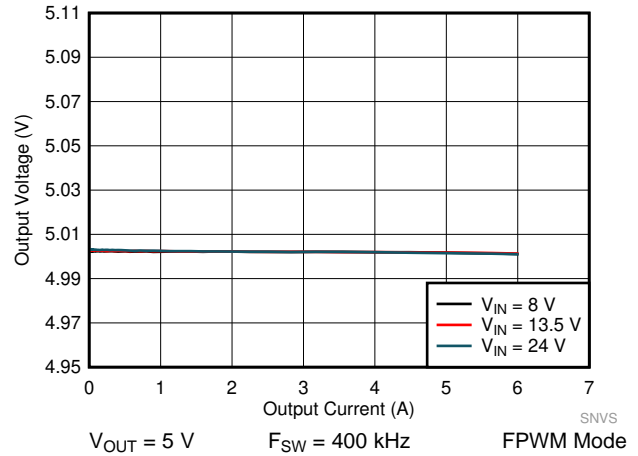
Figure 48. LM61460-Q1 Load and Line Regulation
