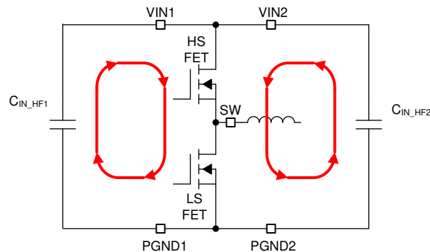
Figure 87. Input Current Loop
