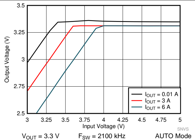
Figure 52. LM61460-Q1 Dropout Curve
