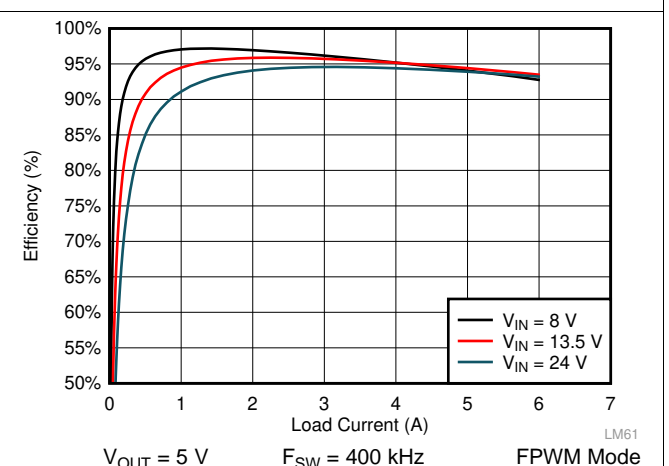
Figure 40. LM61460-Q1 Efficiency
