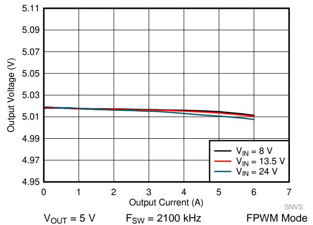
Figure 50. LM61460-Q1 Load and Line Regulation
