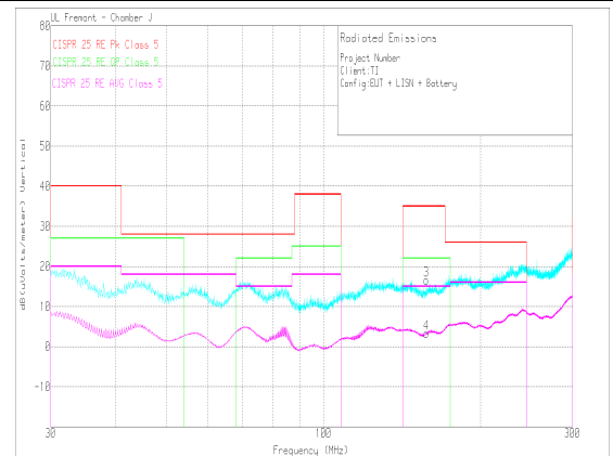
V_{OUT} = 5\text{ V} F_{SW} = 400\text{ kHz} I_{OUT} = 5\text{ A} Frequency Tested: 30 MHz to 300 MHz
