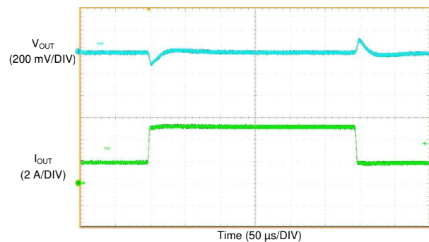
Figure 68. LM61460-Q1 Load Transient
