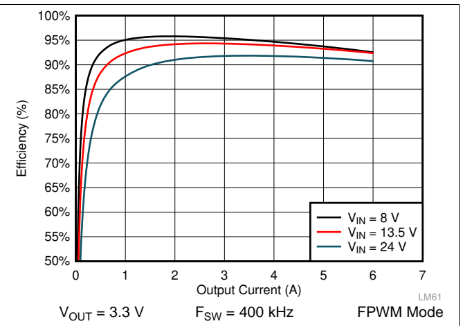
Figure 36. LM61460-Q1 Efficiency
