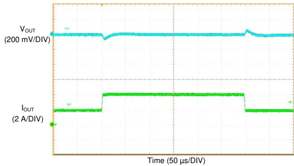
Figure 71. LM61460-Q1 Load Transient
