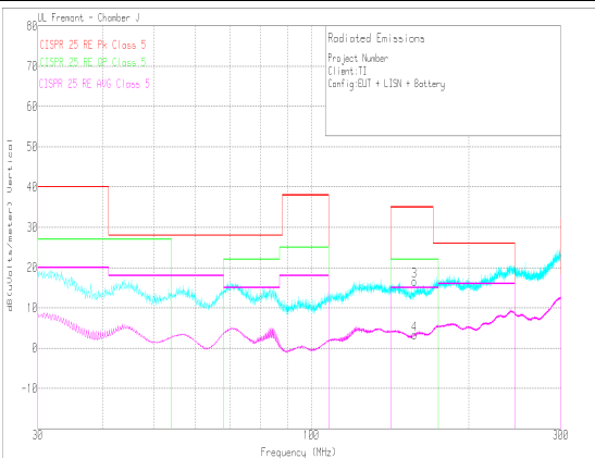
V_{OUT} = 5\text{ V} F_{SW} = 400\text{ kHz} I_{OUT} = 5\text{ A} Frequency Tested: 30 MHz to 300 MHz
