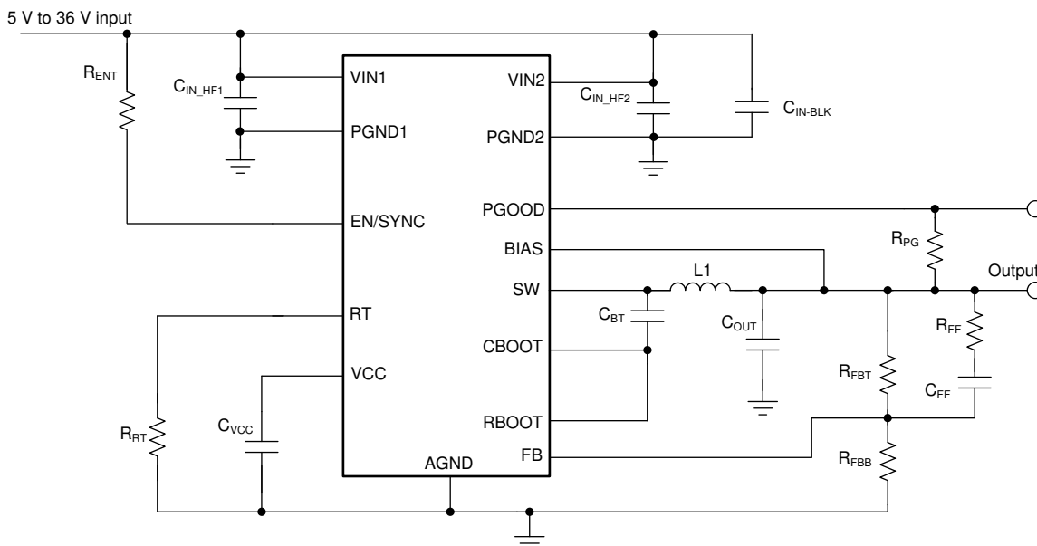
Figure 31. Example Application Circuit
