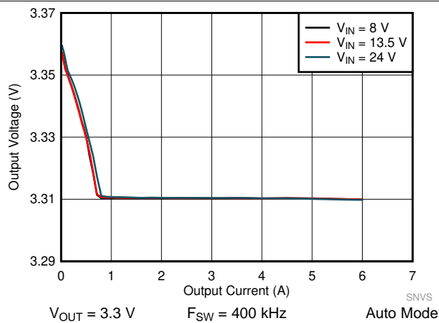
Figure 43. LM61460-Q1 Load and Line Regulation
