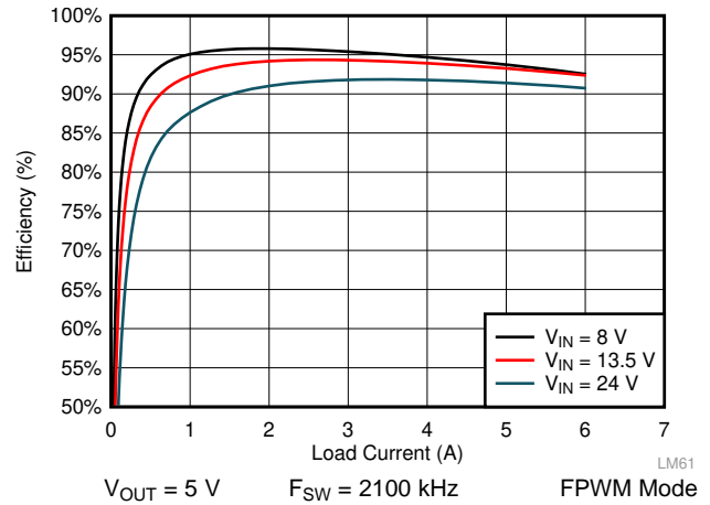
Figure 42. LM61460-Q1 Efficiency
