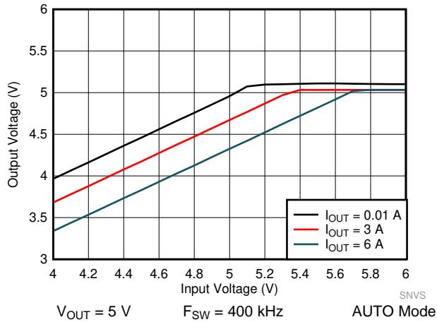
Figure 53. LM61460-Q1 Dropout Curve
