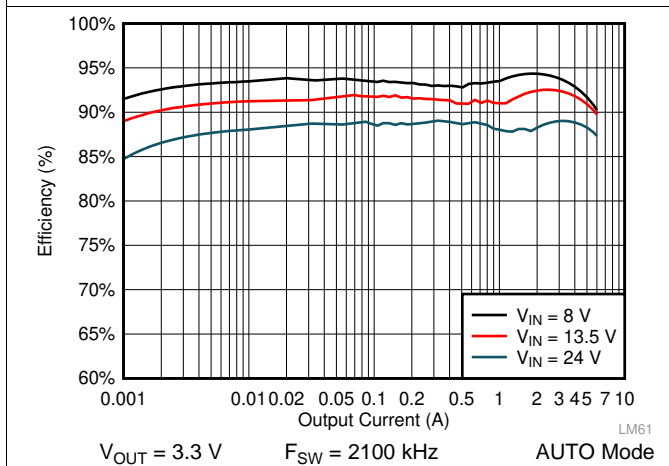
Figure 37. LM61460-Q1 Efficiency
