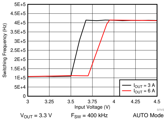
Figure 55. LM61460-Q1 Frequency Dropout
