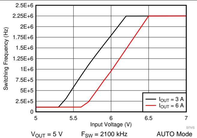
Figure 58. LM61460-Q1 Frequency Dropout Curve
