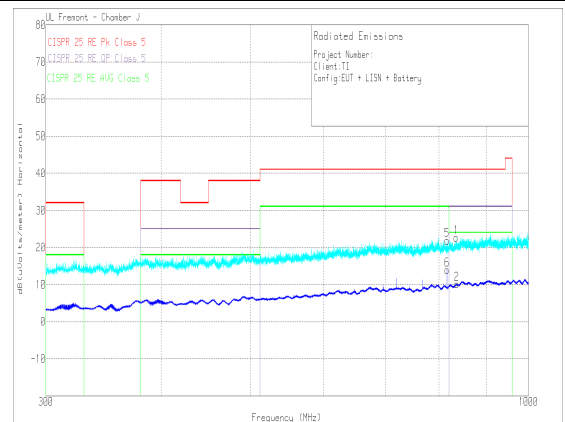
V_{OUT} = 5\text{ V} F_{SW} = 400\text{ kHz} I_{OUT} = 5\text{ A} Frequency Tested: 300 MHz to 1 GHz
