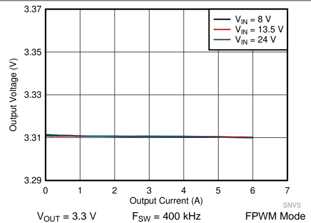
Figure 44. LM61460-Q1 Load and Line Regulation
