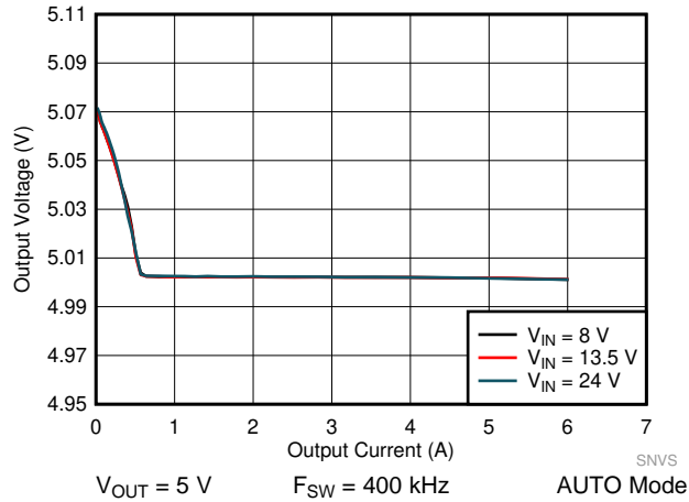
Figure 47. LM61460-Q1 Load and Line Regulation
