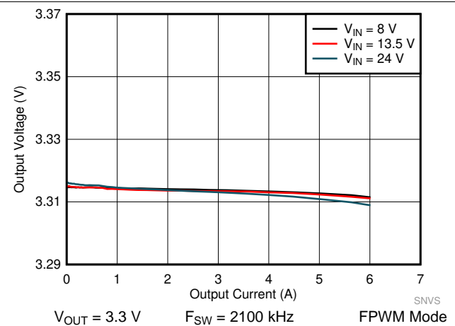
Figure 46. LM61460-Q1 Load and Line Regulation
