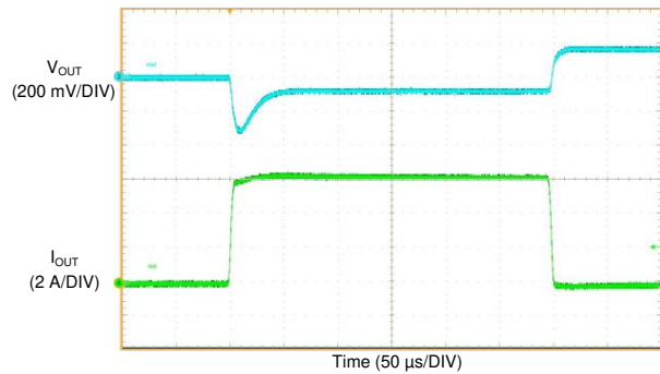
Figure 72. LM61460-Q1 Load Transient
