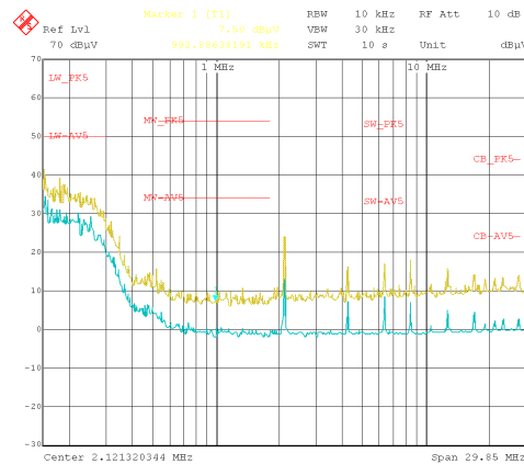
Figure 84. Conducted EMI versus CISPR25 Limits (Yellow: Peak Signal, Blue: Average Signal)
