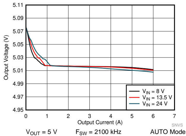
Figure 49. LM61460-Q1 Load and Line Regulation
