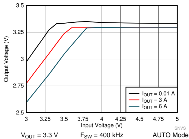
Figure 51. LM61460-Q1 Dropout Curve
