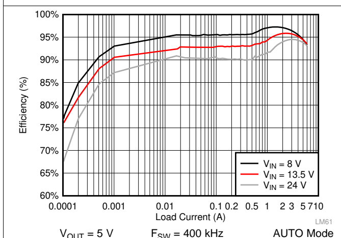
Figure 39. LM61460-Q1 Efficiency
