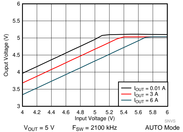
Figure 54. LM61460-Q1 Dropout Curve
