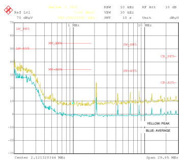
Conducted EMI: V_{OUT} = 5\text{ V} , I_{OUT} = 5\text{ A}
