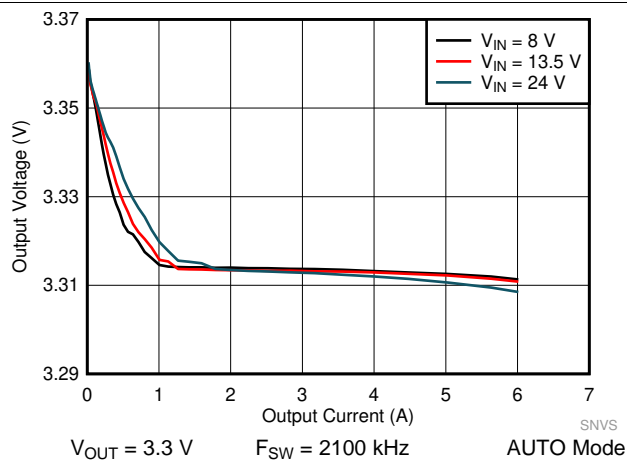
Figure 45. LM61460-Q1 Load and Line Regulation
