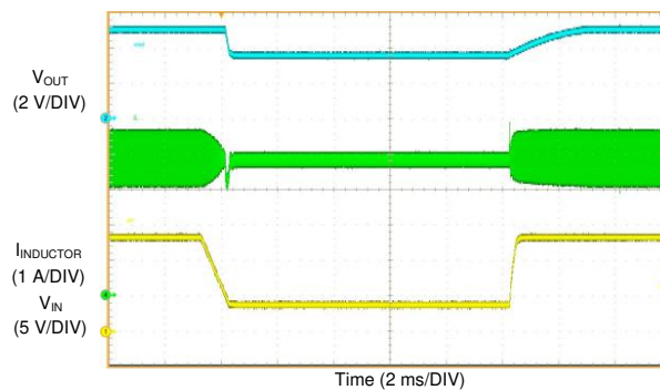
Figure 18. Recovery From Dropout ( V_{OUT} = 5\text{ V} , I_{OUT} = 4\text{ A} , V_{IN} = 13.5\text{ V} to 4\text{ V} to 13.5\text{ V} )
