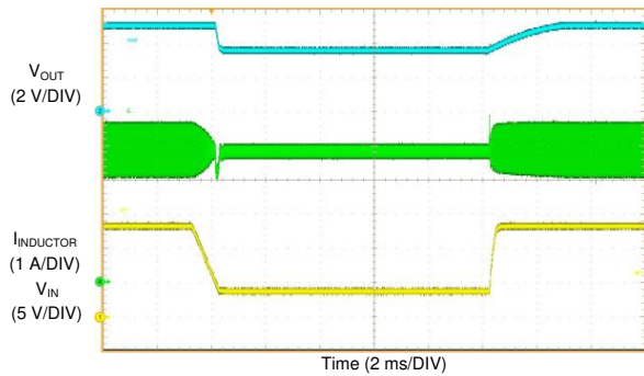
Figure 65. LM61460-Q1 Short Circuit Recovery
