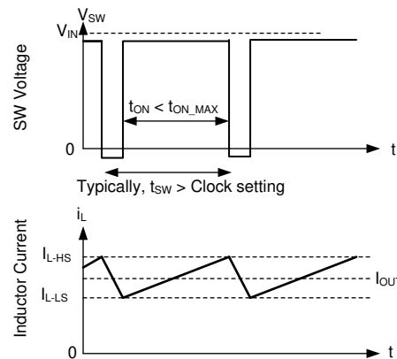
Figure 21. Current Limit Waveforms
