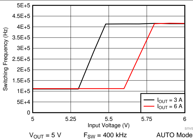
Figure 57. LM61460-Q1 Frequency Dropout Curve
