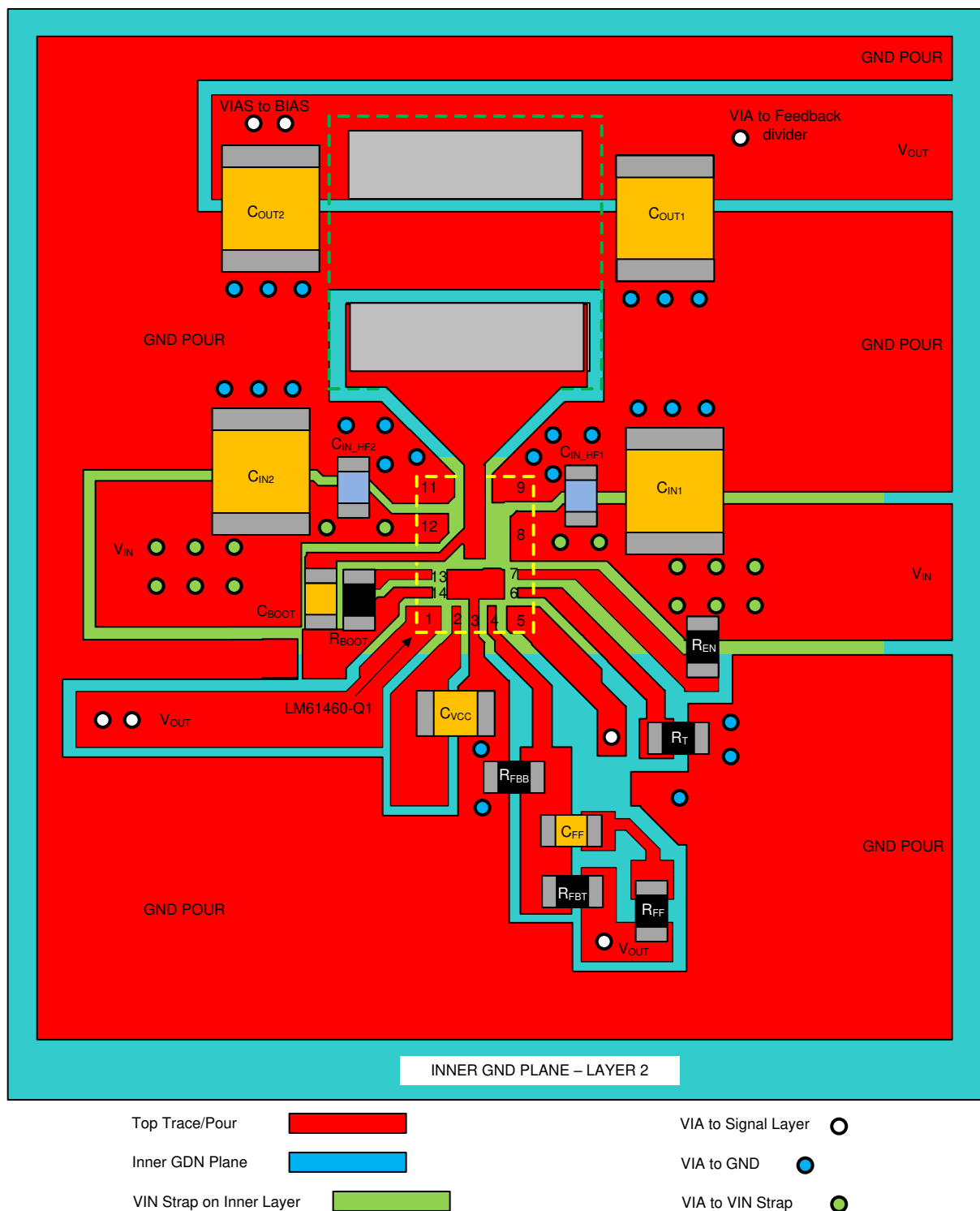
Figure 88. Layout Example
