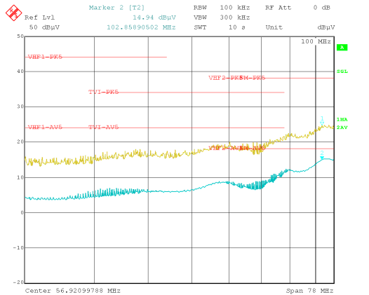
V_{OUT} = 5\text{ V} F_{SW} = 400\text{ kHz} I_{OUT} = 5\text{ A} Frequency Tested: 30 MHz to 108 MHz
