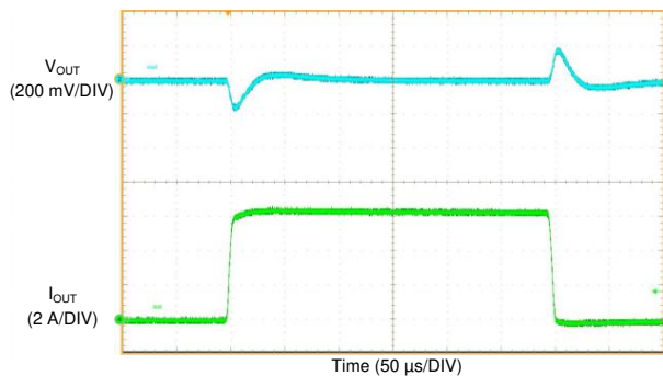
Figure 73. LM61460-Q1 Load Transient
