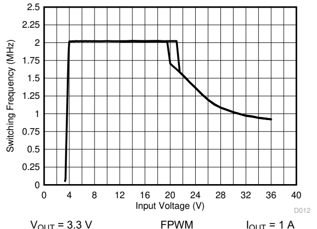
Figure 9-28. Switching Frequency vs Input Voltage
