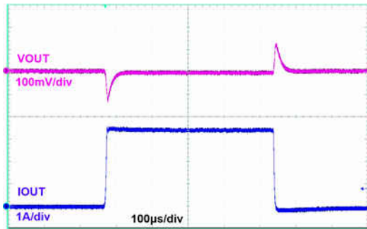
FPWM V_{OUT} = 3.3\text{ V} L = 2.2\ \mu\text{H} , C_{OUT} = 3 \times 22\ \mu\text{F} I_{OUT} = 0\text{ A to } 3.5\text{ A} T_R = T_F = 1\ \mu\text{s}
