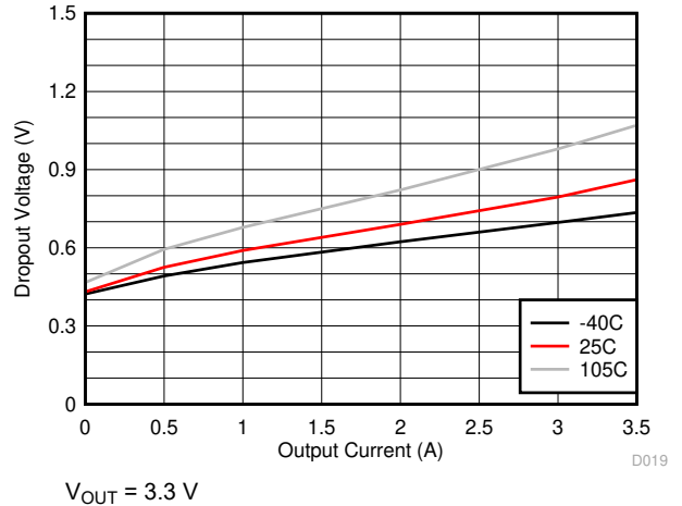
Figure 9-26. Dropout for \geq 1.85\text{ MHz}
