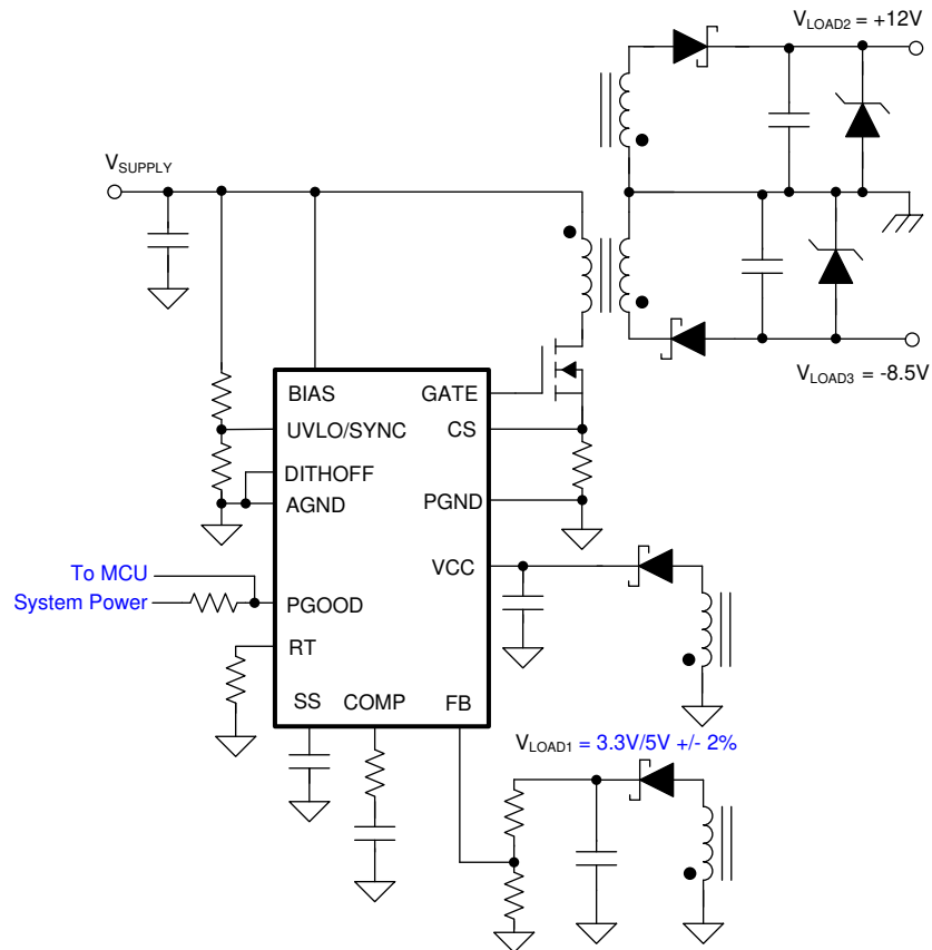
Figure 10-11. Primary-Side Regulated Multiple-Output Isolated Flyback
