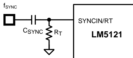
Figure 28. Oscillator Synchronization Through AC Coupling
