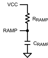
Figure 38. R_{RAMP} to VCC for V_{OUT} > 7.5 V
