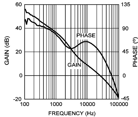
Figure 37. Overall Voltage Loop Gain and Phase
