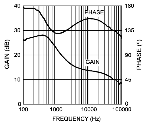
Figure 36. Error Amplifier Gain and Phase
