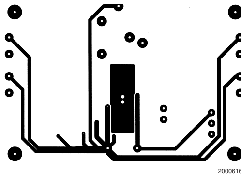
FIGURE 9. Recommended LD PC Board Layout: Bottom Layer
