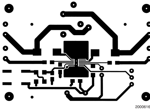
FIGURE 8. Recommended LD PC Board Layout: TOP Top Layer
