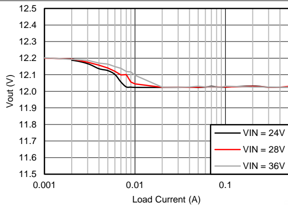
Figure 85. Output Voltage Regulation
