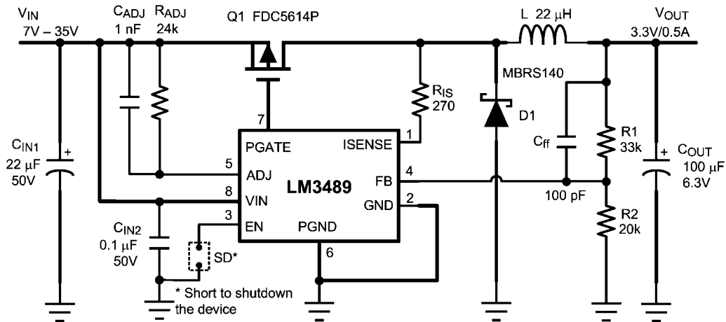
FIGURE 7. Typical Application Schematic for V_{OUT} = 3.3\text{V}/500\text{mA}
