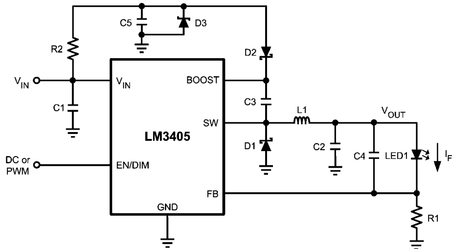
FIGURE 17. V_{BOOST} derived from V_{IN} through a Shunt Zener Diode (D3) ( V_{IN} = 15V , I_F = 1A )
