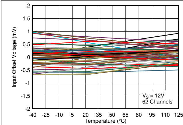
Figure 3-15. Input Offset Voltage vs. Temperature at 12V
