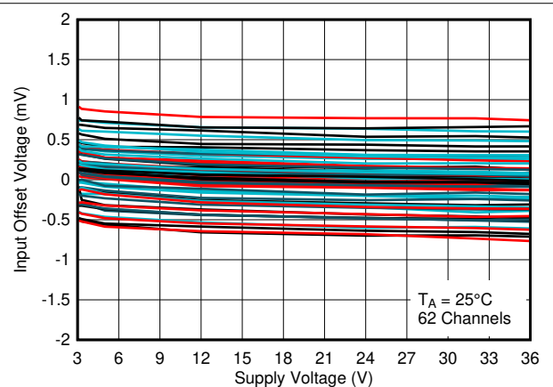
Figure 6-12. Input Offset Voltage vs. Supply Voltage at 25°C
