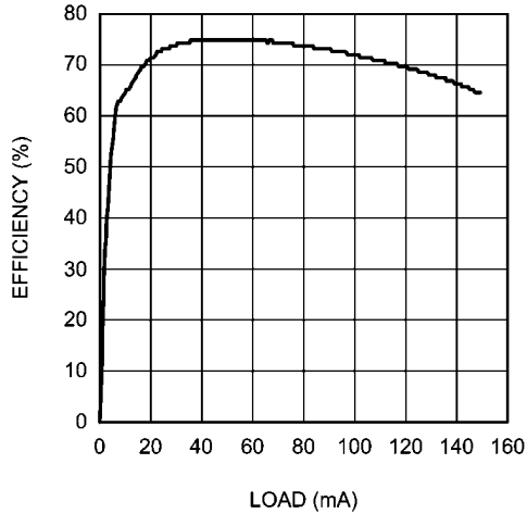
Efficiency vs Load Current - "X" V_{IN} = 3.3V, V_{OUT} = 12V
