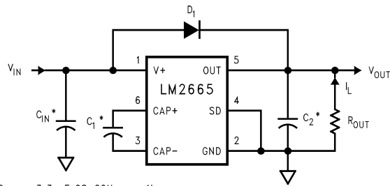
FIGURE 1. LM2665 Test Circuit
