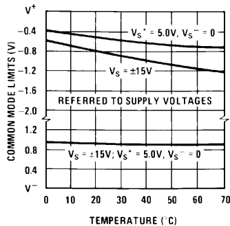
Figure 23. Common-Mode Limits
