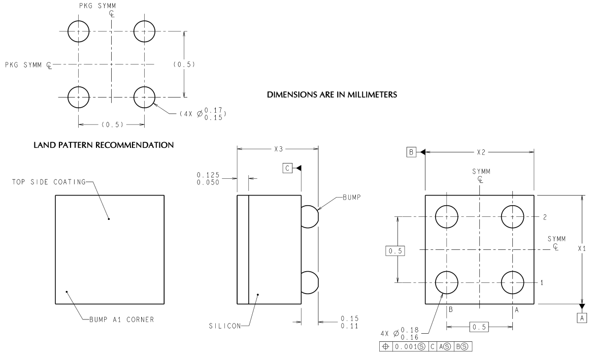
4-Bump Thin micro SMD Ball Grid Array Package (Small Bump) Order Number LM20SITP or LM20SITPX NS Package Number TPA04EEA The following dimensions apply to the TPA04EEA package shown above: X1 = X2 = 879µm ±30µm X3 = 500µm ±75µm
