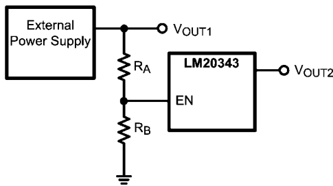
FIGURE 5. Sequencing LM20343 with Precision Enable
