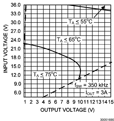
FIGURE 8. Safe Thermal Operating Areas ( I_{OUT} = 3A , f_{SW} = 350kHz )
