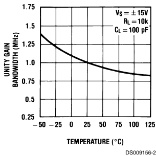
Gain Bandwidth
