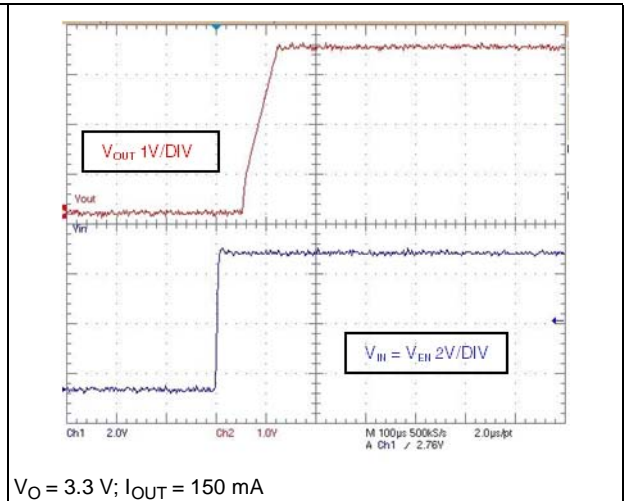
Figure 23. Startup transient
