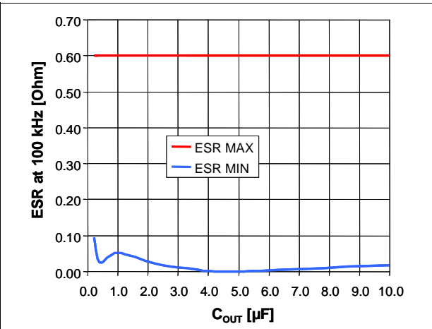
Figure 15. Stability area
