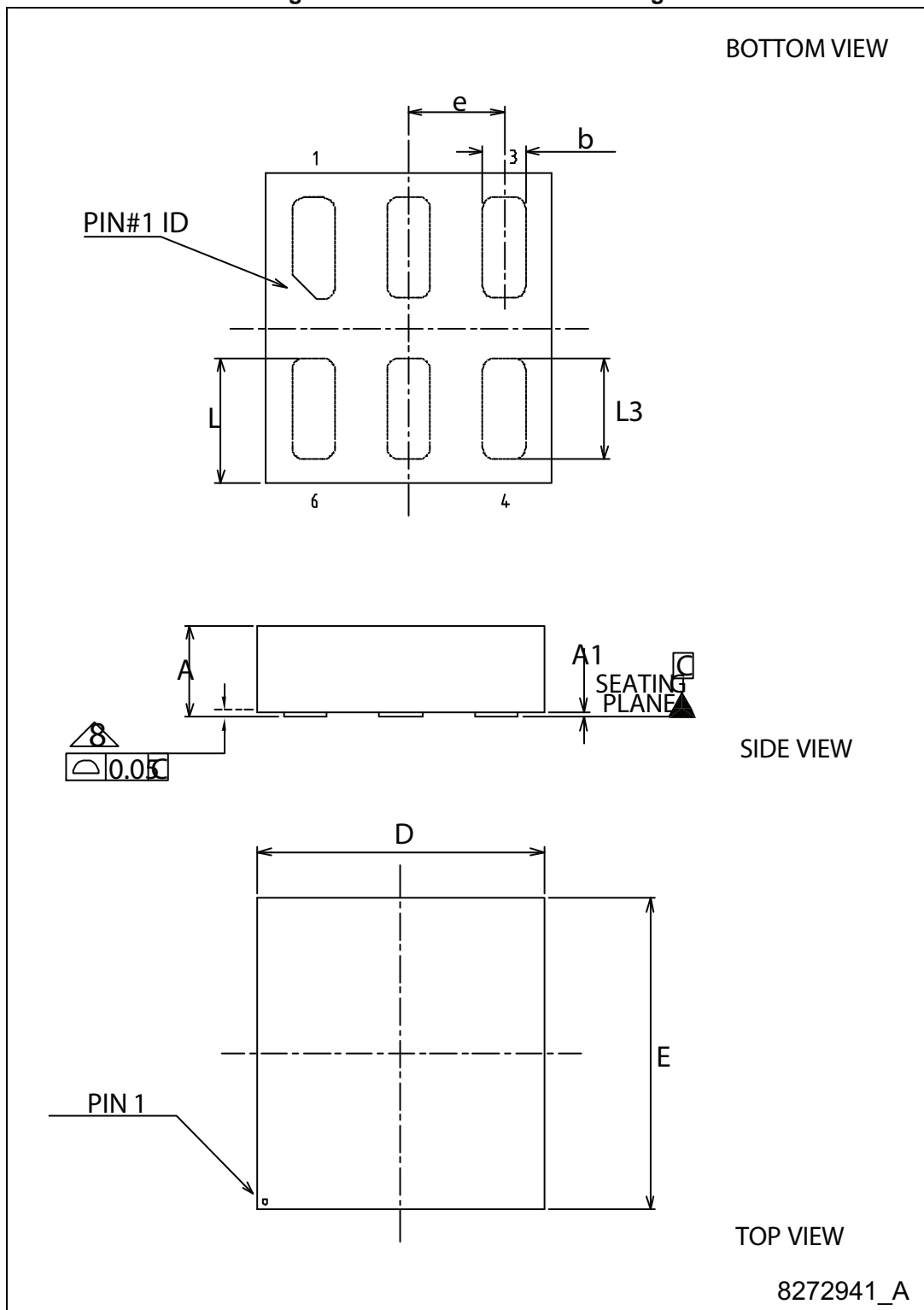
Figure 49. DFN6 1.2x1.3 mm drawing
