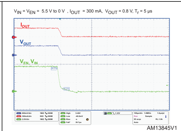
Figure 40. Turn-off time
