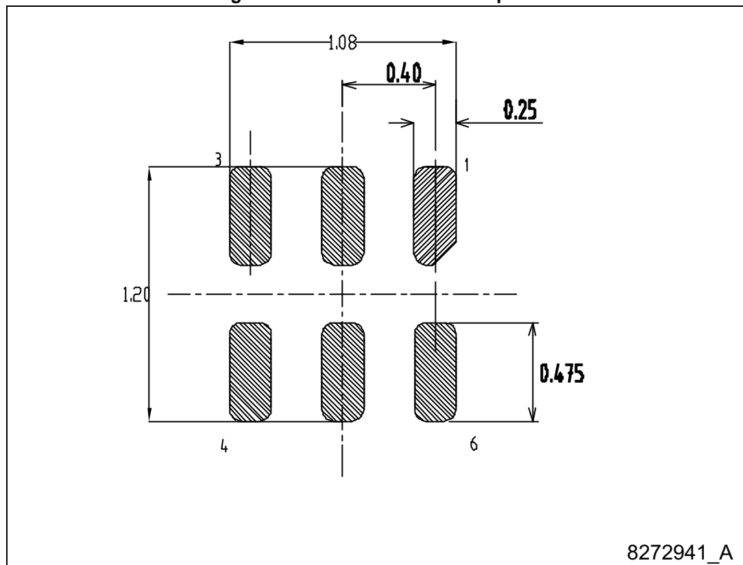
Figure 50. DFN6 1.2x1.3 mm footprint
