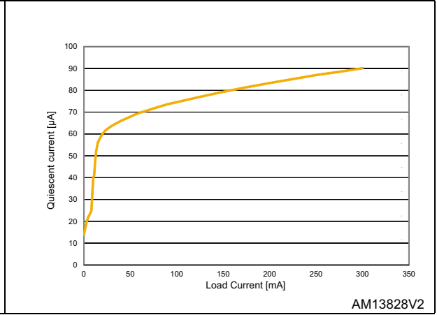
Figure 22. Quiescent current vs. load current (normal mode)
