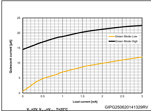
Figure 23. Quiescent current vs. load current (light load)
