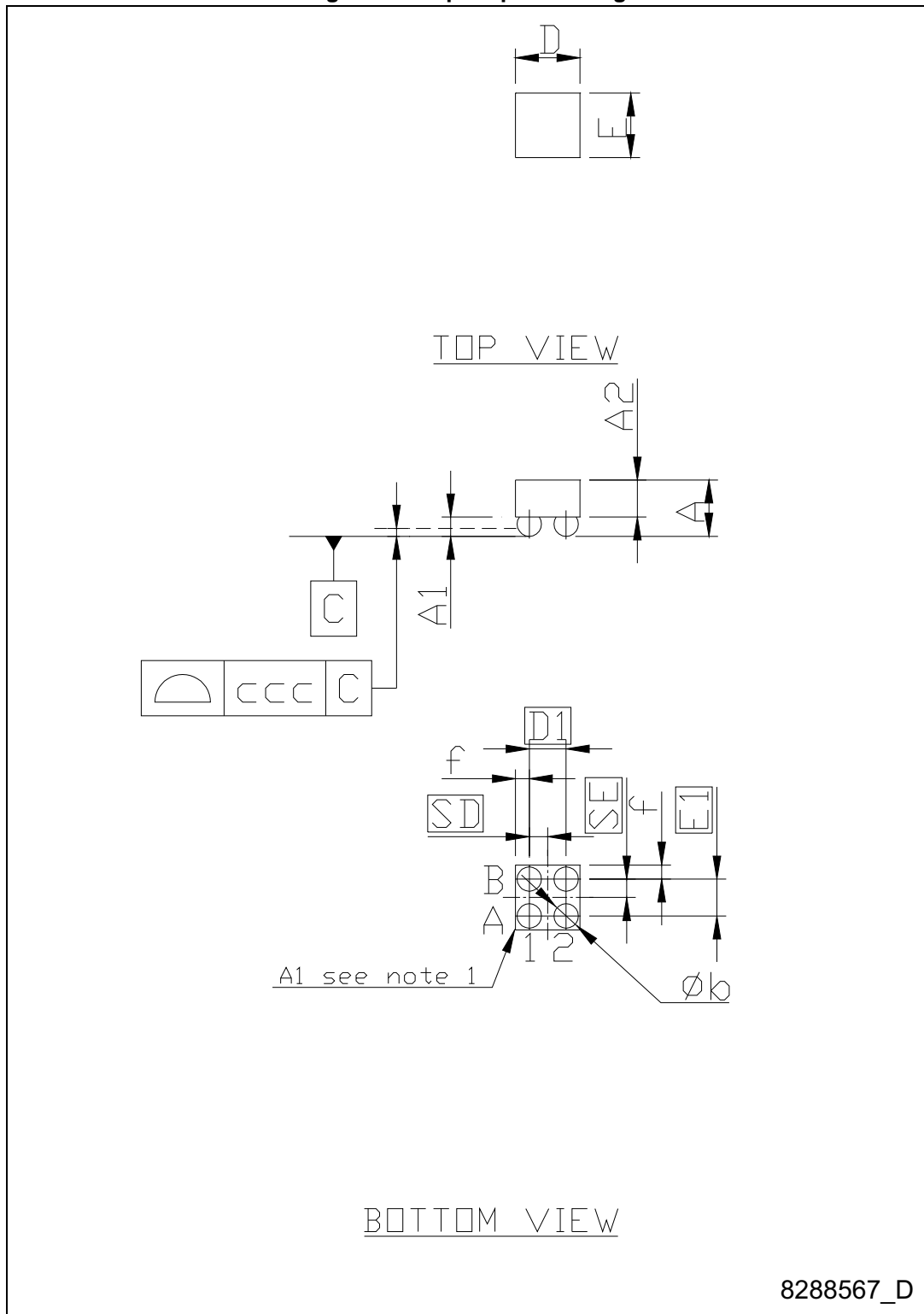
Figure 47. Flip-chip 4 drawing
