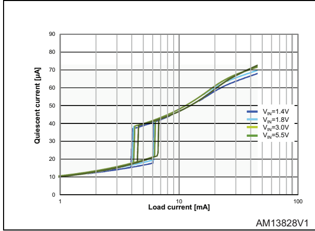
Figure 21. Quiescent current vs. output current (auto green mode)
