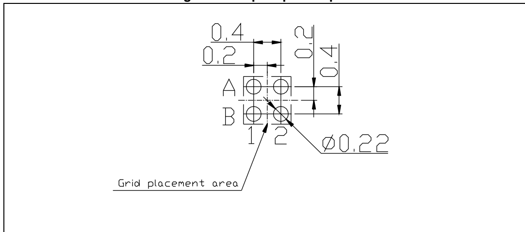
Figure 37. Flip-chip 4 footprint
