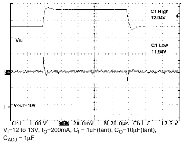
Figure 18 : Line Transient
