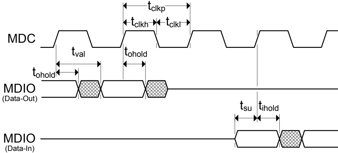
Figure 5.9 SMI Timing
