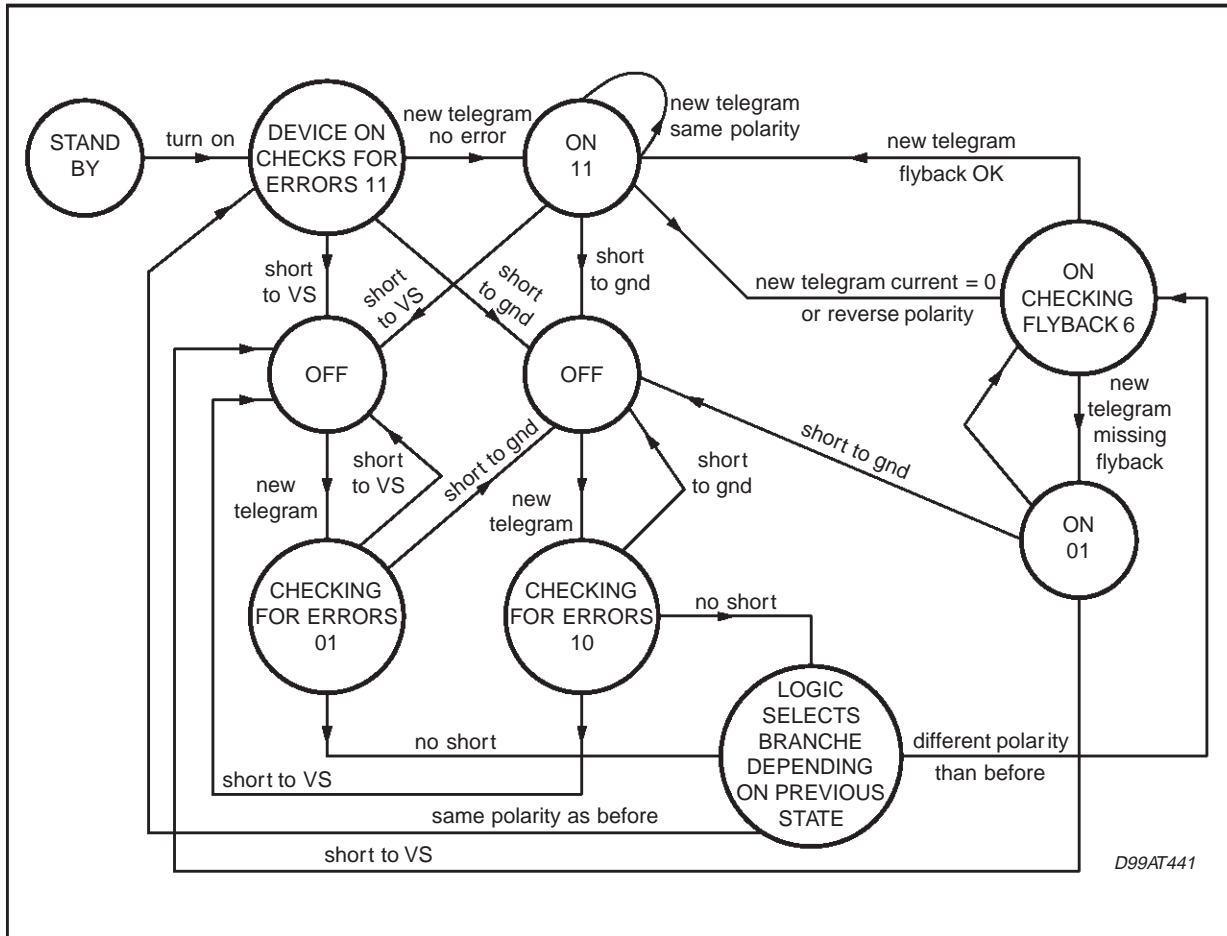
Figure 11. State diagram.
