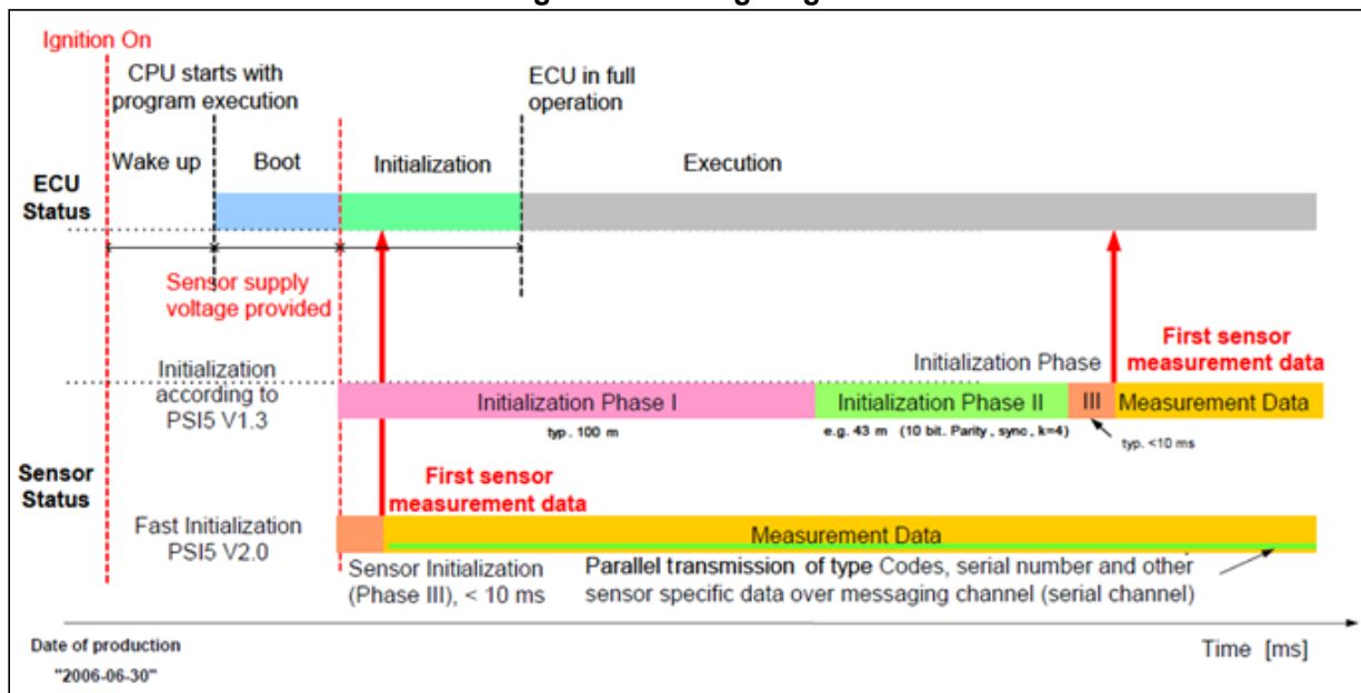
Figure 19. Timing diagram
