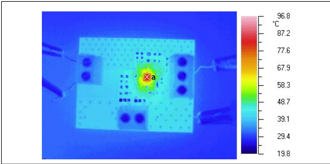
Figure 24. Thermal image of the demo board
