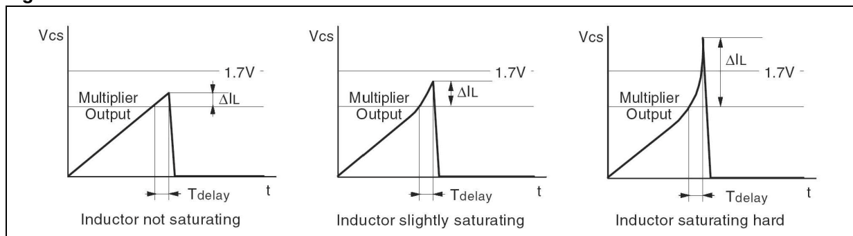
Figure 39. Effect of boost inductor saturation on the MOSFET current and detection method
