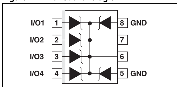
Figure 1. Functional diagram
