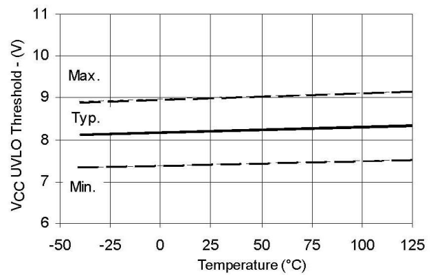
Figure 21B. V_{CC}/V_{BS} Undervoltage Threshold(-) vs. Temperature
