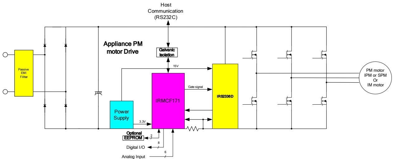
Figure 1. Typical Application Block Diagram Using IRMCF171
