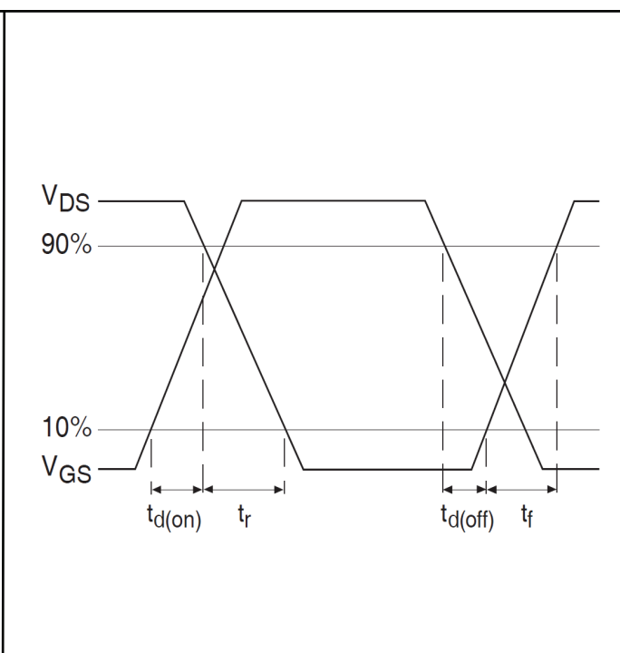
Figure 20b Switching Time Waveforms
