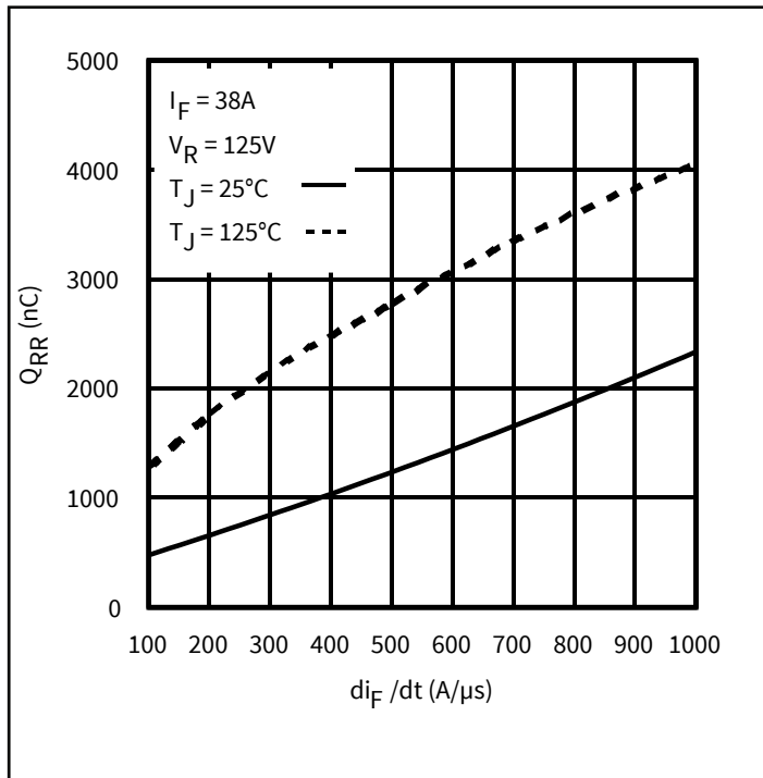
Figure 20 Typical Stored Charge vs. di/dt
