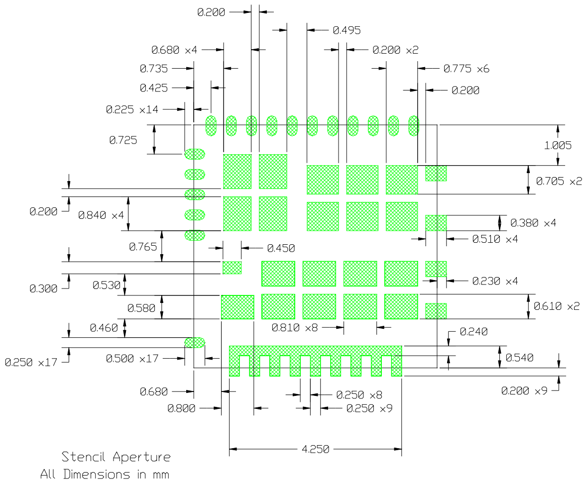
Figure 35: Stencil design
