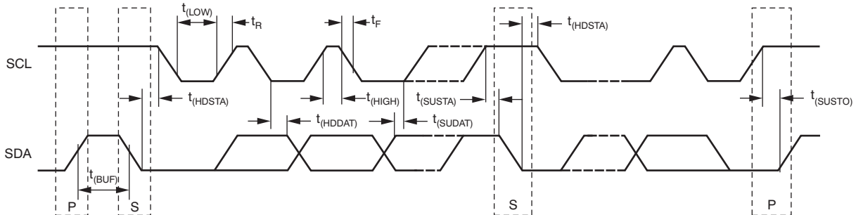
Figure 28. Bus Timing Diagram
