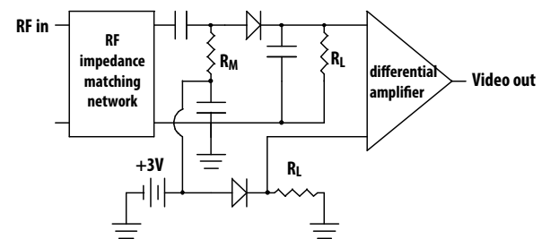
Figure 13. Differential Detector.
