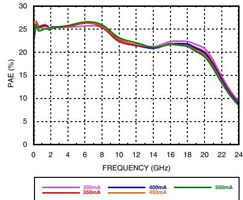
PAE @ Psat vs. Idq
