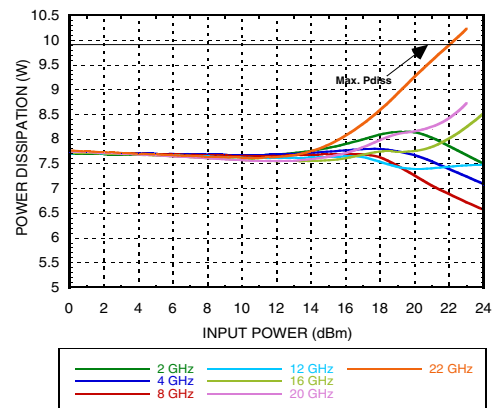
Power Dissipation @ 85C
